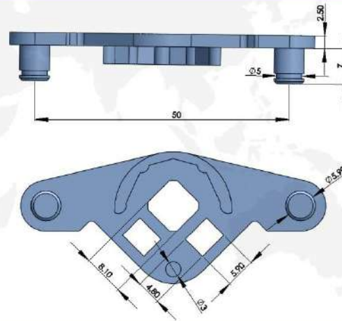
316 不锈钢连接件 316 STAINLESS STEEL FITTINGS
