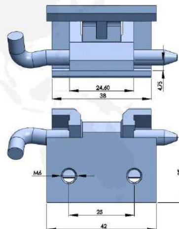
316不锈钢铰链 316 STAINLESS STEEL HINGE
