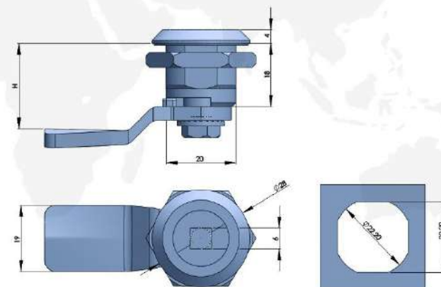
316不锈钢转舌锁 316 STAINLESS STEEL QUARTER TURN
