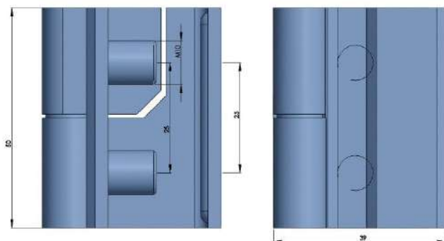
316不锈钢铰链 316 STAINLESS STEEL HINGE
