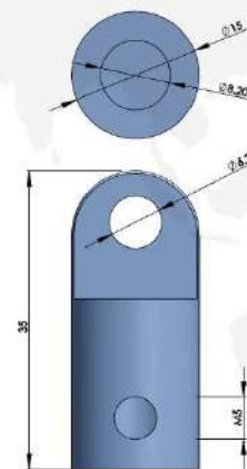
316 不锈钢连接件 316 STAINLESS STEEL FITTINGS
