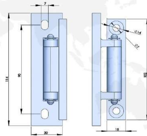
316不锈钢铰链 316 STAINLESS STEEL HINGE
