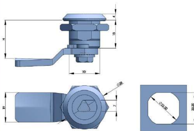
316不锈钢转舌锁 316 STAINLESS STEEL QUARTER TURN
