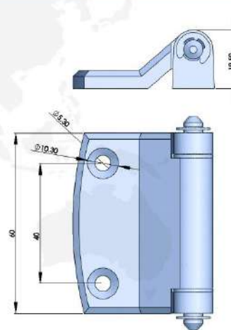
316不锈钢铰链 316 STAINLESS STEEL HINGE
