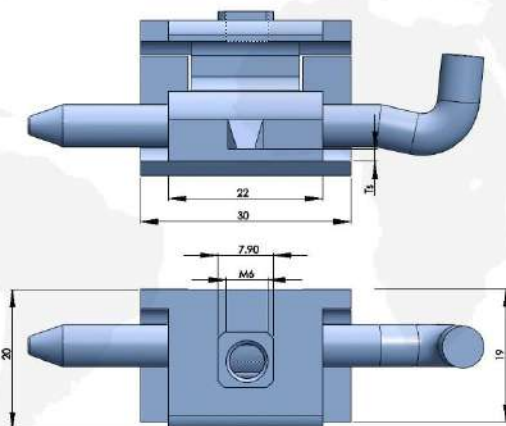
316不锈钢铰链 316 STAINLESS STEEL HINGE
