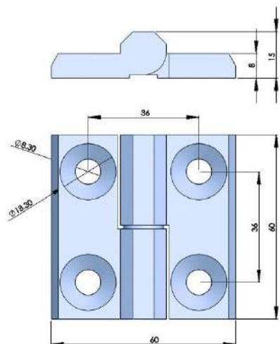
316不锈钢合页 316 STAINLESS STEEL HINGE
