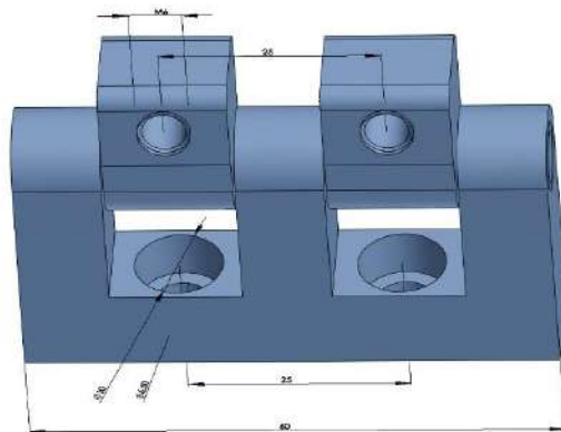
316不锈钢铰链 316 STAINLESS STEEL HINGE
