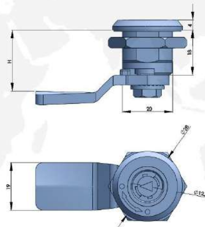
316不锈钢转舌锁 316 STAINLESS STEEL QUARTER TURN
