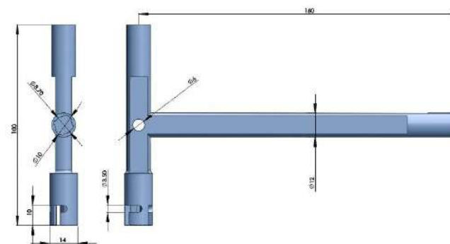
316 不锈钢钥匙 316 STAINLESS STEEL KEY
