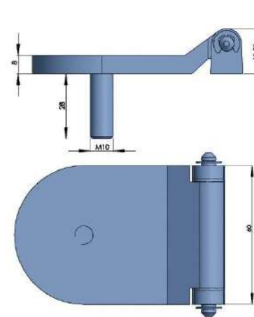
316不锈钢铰链 316 STAINLESS STEEL HINGE
