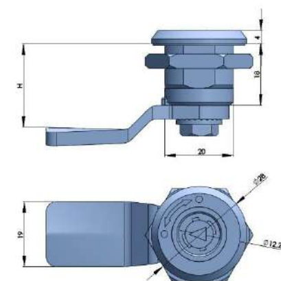
316不锈钢转舌锁 316 STAINLESS STEEL QUARTER TURN
