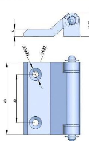
316不锈钢铰链 316 STAINLESS STEEL HINGE
