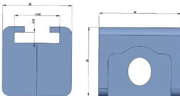
316 不锈钢连接件 316 STAINLESS STEEL FITTINGS
