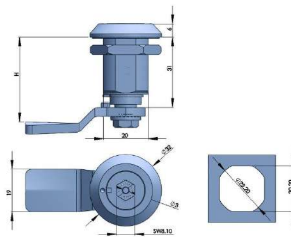
316不锈钢压紧锁 COMPRESSION LATCH AISI316
