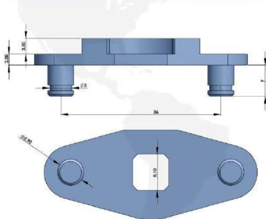
316 不锈钢连接件 316 STAINLESS STEEL FITTINGS
