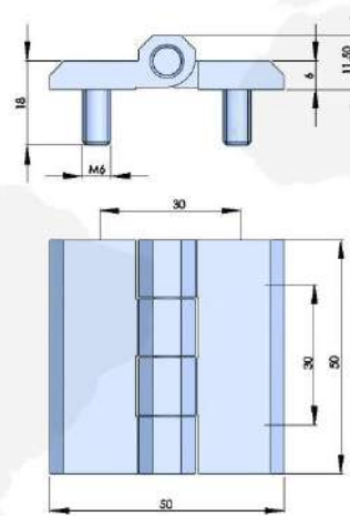
316不锈钢合页 316 STAINLESS STEEL HINGE
