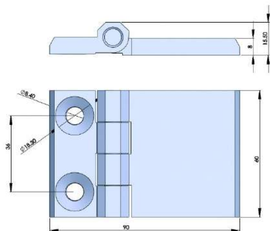
316不锈钢合页 316 STAINLESS STEEL HINGE
