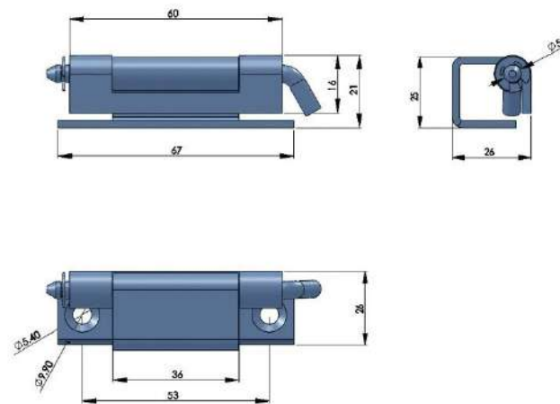
316不锈钢铰链 316 STAINLESS STEEL HINGE
