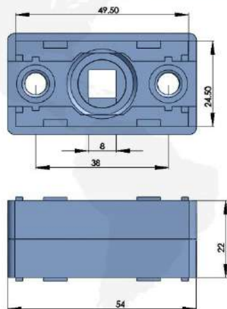
316 不锈钢连接件 316 STAINLESS STEEL FITTINGS
