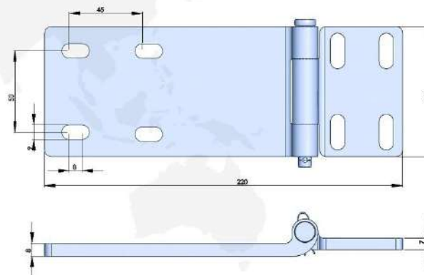
316不锈钢合页 316 STAINLESS STEEL HINGE
