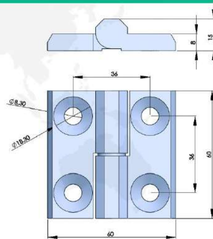
316不锈钢合页 316 STAINLESS STEEL HINGE
