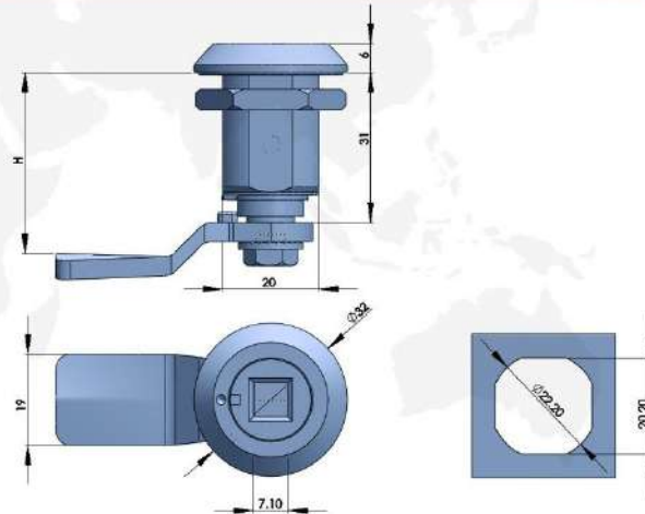
316不锈钢压紧锁 COMPRESSION LATCH AISI316
