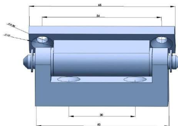
316不锈钢铰链 316 STAINLESS STEEL HINGE
