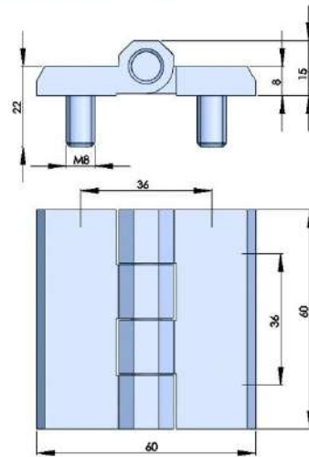
316不锈钢合页 316 STAINLESS STEEL HINGE
