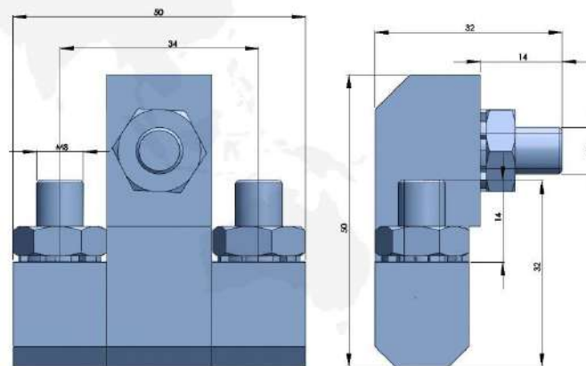
316不锈钢铰链 316 STAINLESS STEEL HINGE
