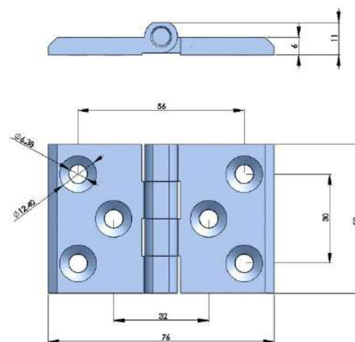
316不锈钢合页 316 STAINLESS STEEL HINGE
