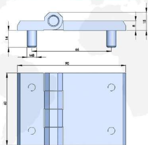
316不锈钢合页 316 STAINLESS STEEL HINGE
