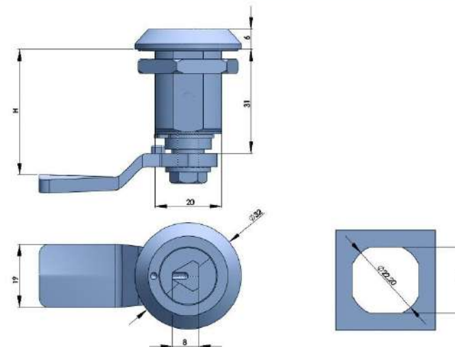
316不锈钢压紧锁 COMPRESSION LATCH AISI316
