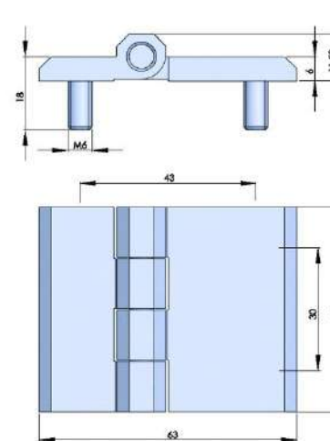
316不锈钢合页 316 STAINLESS STEEL HINGE
