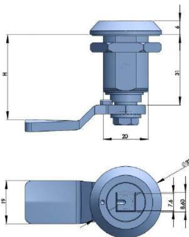
316不锈钢压紧锁 COMPRESSION LATCH AISI316
