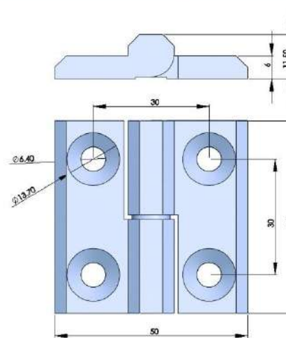
316不锈钢合页 316 STAINLESS STEEL HINGE
