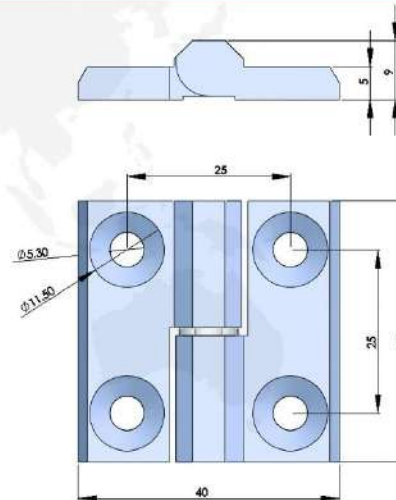
316不锈钢合页 316 STAINLESS STEEL HINGE
