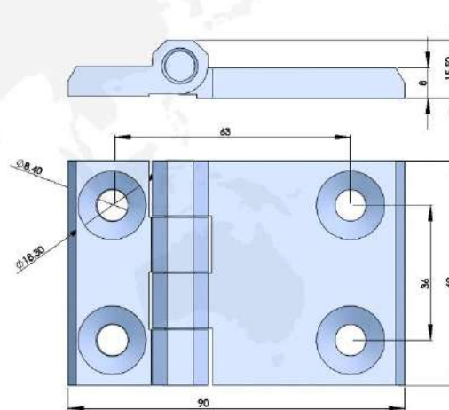
316不锈钢合页 316 STAINLESS STEEL HINGE
