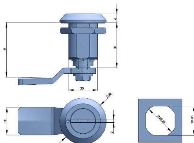
316不锈钢压紧锁 COMPRESSION LATCH AISI316
