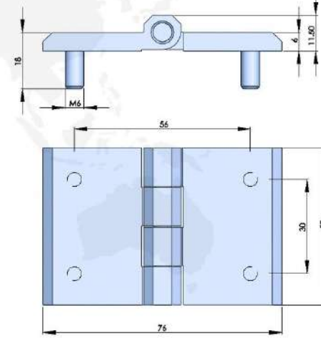
316不锈钢合页 316 STAINLESS STEEL HINGE
