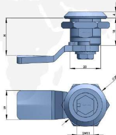
316不锈钢转舌锁 316 STAINLESS STEEL QUARTER TURN
