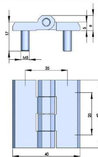
316不锈钢合页 316 STAINLESS STEEL HINGE
