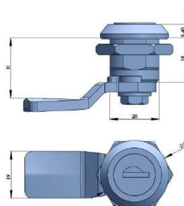
316不锈钢转舌锁 316 STAINLESS STEEL QUARTER TURN
