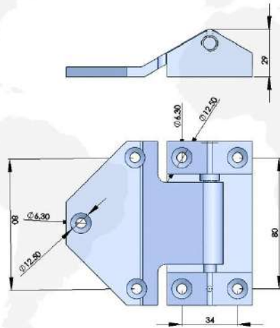
316不锈钢铰链 316 STAINLESS STEEL HINGE
