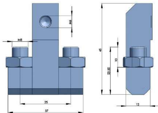
316不锈钢铰链 316 STAINLESS STEEL HINGE
