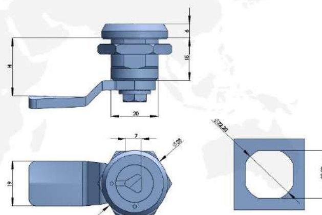
316安全转舌锁 316 SECURITY QUARTER TURN
