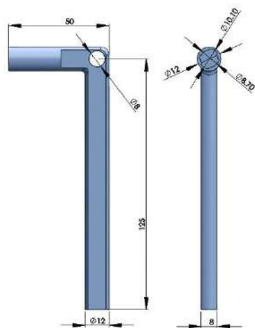
316 不锈钢钥匙 316 STAINLESS STEEL KEY
