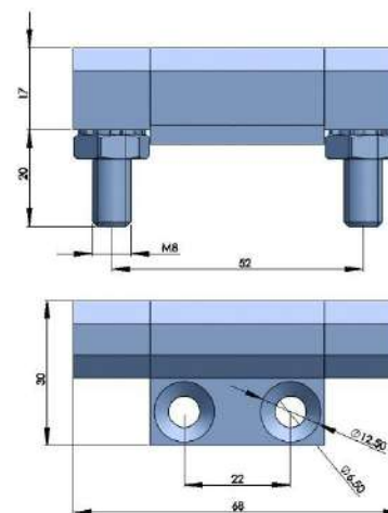
316不锈钢铰链 316 STAINLESS STEEL HINGE
