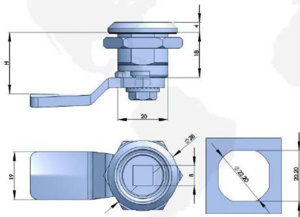
316不锈钢转舌锁 316 STAINLESS STEEL QUARTER TURN
