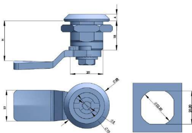
316不锈钢转舌锁 316 STAINLESS STEEL QUARTER TURN
