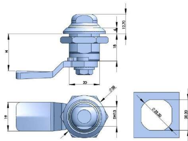
316不锈钢转舌锁 316 STAINLESS STEEL QUARTER TURN
