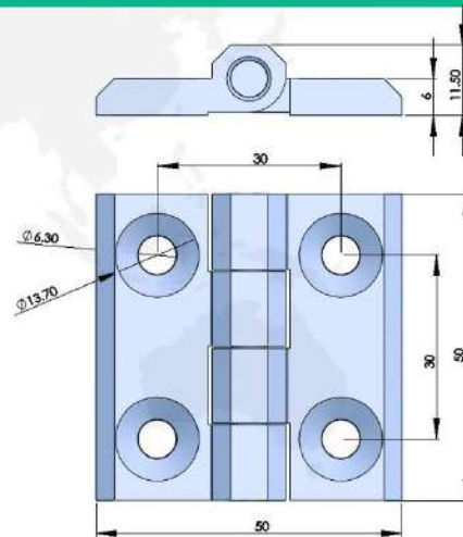
316不锈钢合页 316 STAINLESS STEEL HINGE
