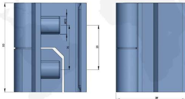
316不锈钢铰链 316 STAINLESS STEEL HINGE
