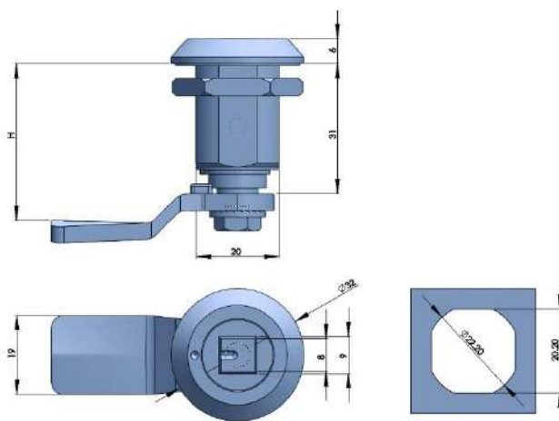
316不锈钢压紧锁 COMPRESSION LATCH AISI316
