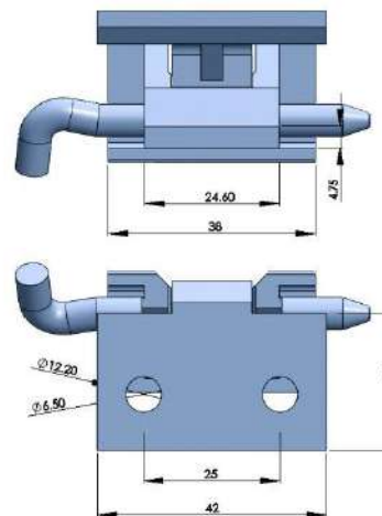
316不锈钢铰链 316 STAINLESS STEEL HINGE
