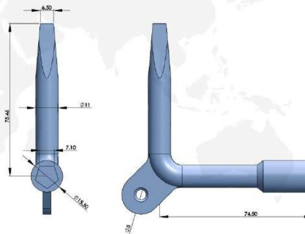
316 不锈钢钥匙 316 STAINLESS STEEL KEY
