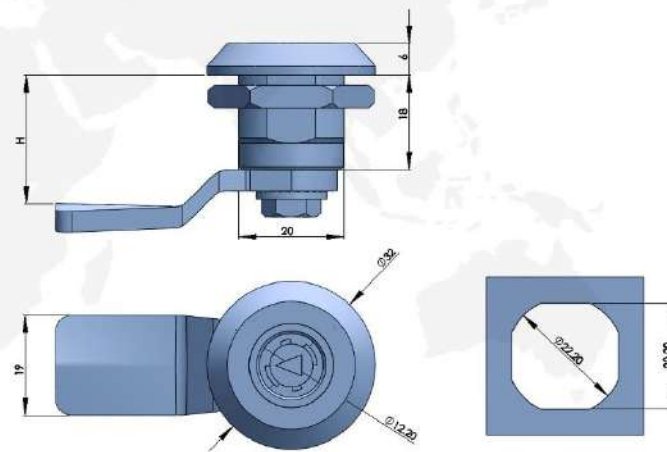
316不锈钢压紧锁 COMPRESSION LATCH AISI316
