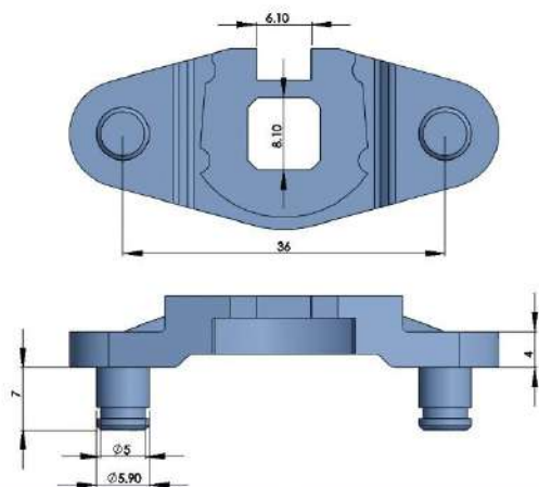
316 不锈钢连接件 316 STAINLESS STEEL FITTINGS
