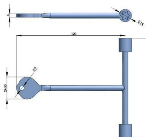
316 不锈钢钥匙 316 STAINLESS STEEL KEY
