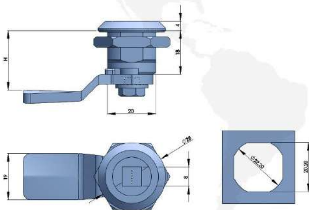
316不锈钢转舌锁 316 STAINLESS STEEL QUARTER TURN
