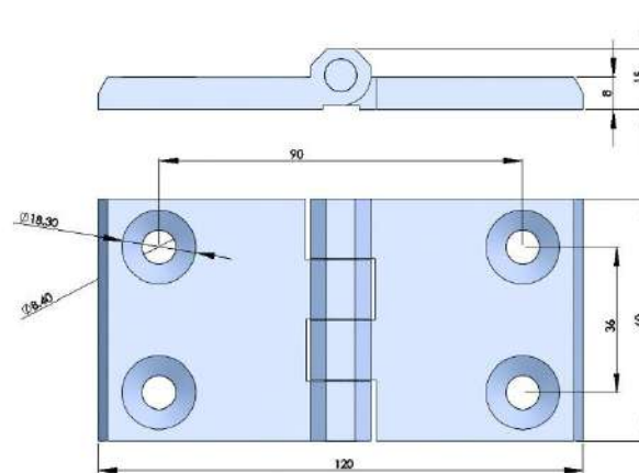
316不锈钢合页 316 STAINLESS STEEL HINGE
