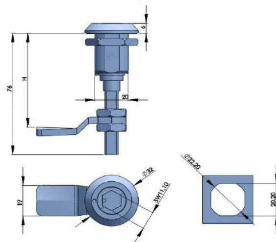
316不锈钢压紧锁 COMPRESSION LATCH AISI316
