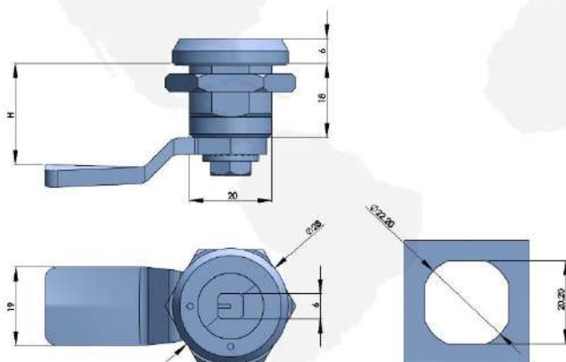
316安全转舌锁 316 SECURITY QUARTER TURN
