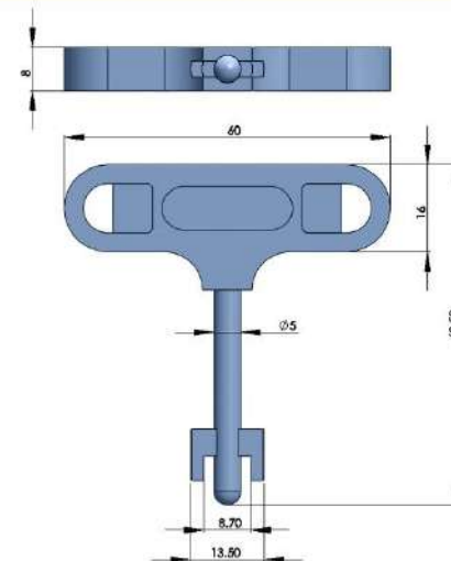
316 不锈钢钥匙 316 STAINLESS STEEL KEY
