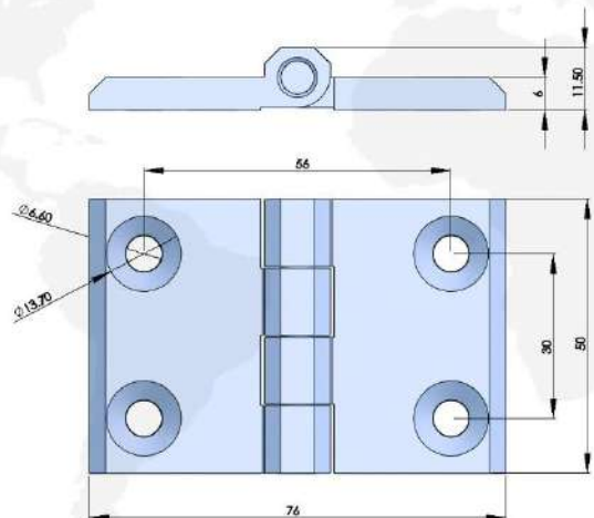
316不锈钢合页 316 STAINLESS STEEL HINGE
