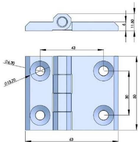
316不锈钢合页 316 STAINLESS STEEL HINGE
