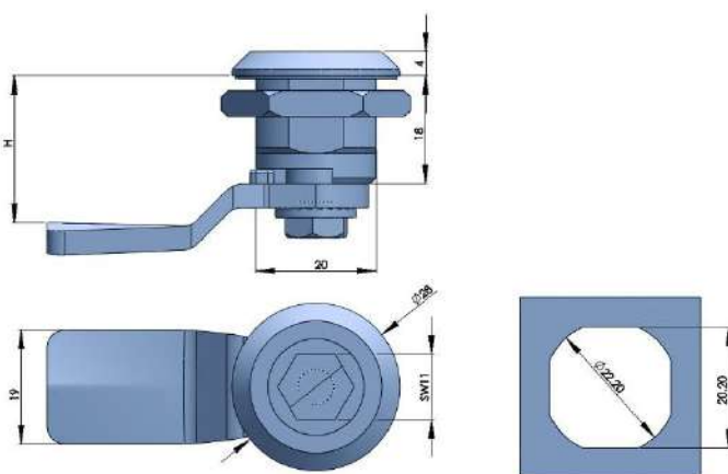
316不锈钢转舌锁 316 STAINLESS STEEL QUARTER TURN
