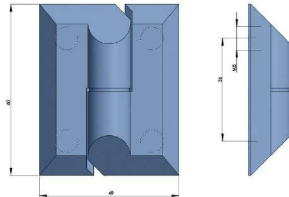
316不锈钢铰链 316 STAINLESS STEEL HINGE
