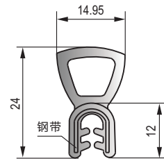
MFT-019 黑色三元乙丙钢带密封条 Black EPDM sealing strip(with steel sheet )
