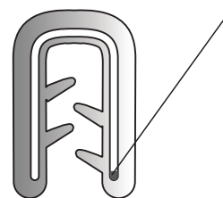
钢丝编织带 Wire Carrier
