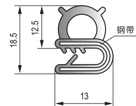
黑色三元乙丙钢带密封条 Black EPDM sealing strip(with steel sheet )
