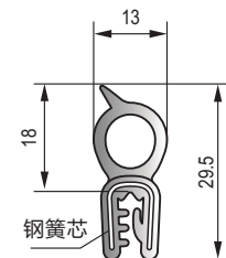
MF-018 黑色三元乙丙钢丝胶条 Black EPDM steel wire strip
