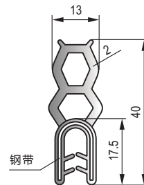
MFT-022 黑色三元乙丙钢带密封条 Black EPDM sealing strip(with steel sheet )
