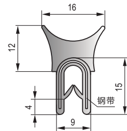
MFT-021 黑色三元乙丙钢带密封条 Black EPDM sealing strip(with steel sheet )
