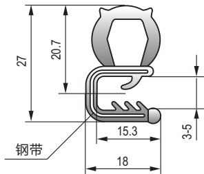
MFT-014 黑色三元乙丙钢带密封条 Black EPDM sealing strip(with steel sheet )
