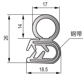
MFT-015 黑色三元乙丙钢带密封条 Black EPDM sealing strip(with steel sheet )
