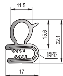
黑色三元乙丙钢带密封条 Black EPDM sealing strip(with steel sheet )
