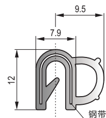
MFT-018 黑色三元乙丙钢带密封条 Black EPDM sealing strip(with steel sheet )
