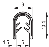
MF-030 PVC橡塑装饰条 PVC trim strip
