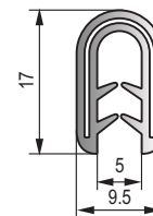
MF-022 PVC橡塑装饰条 PVC trim strip
