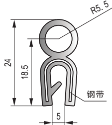
MFT-017 黑色三元乙丙钢带密封条 Black EPDM sealing strip(with steel sheet )
