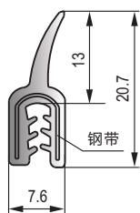
黑色三元乙丙钢带密封条 Black EPDM sealing strip(with steel sheet )
