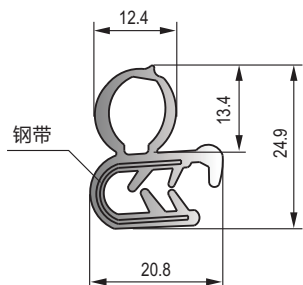
MFT-013 黑色三元乙丙钢带密封条 Black EPDM sealing strip(with steel sheet )
