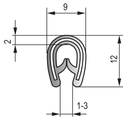
MF-026 PVC橡塑装饰条 PVC trim strip
