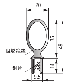
MFT-023 黑色三元乙丙钢片密封条 Black EPDM sealing strip(with steel sheet )
