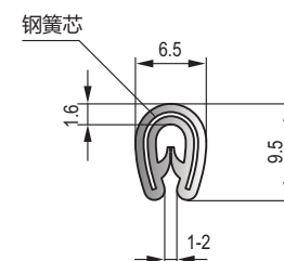
MF-024 PVC橡塑装饰条 PVC trim strip
