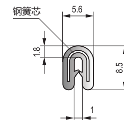
MF-023 PVC橡塑装饰条 PVC trim strip
